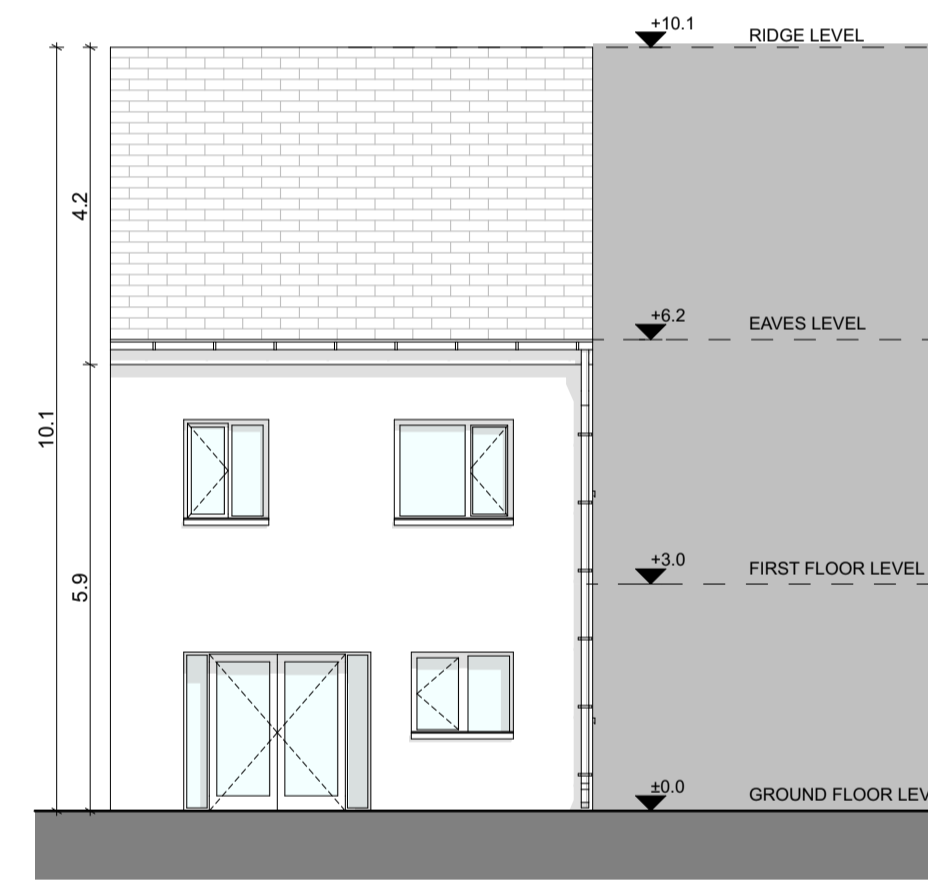
Rear Elevation SCALE 1:100
