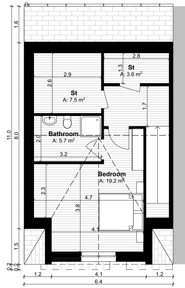
Second Floor Plan SCALE 1:100
